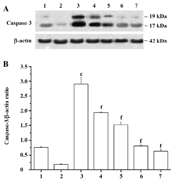
Figure 6. Effects of PCF on the UV-induced caspase-3 activation. HaCaT cells were pretreated with different concentrations of PCF, 20 \mu mol/L SP600125, or 5.68 mmol/L vitamin C for 2 h at 37 °C before UV irradiation. Nine hours after UV irradiation, the cells were harvested and assayed for the expression of cleaved caspases-3. Results presented are the mean \pm SD from 3 independent experiments. Expression of \beta -actin is shown for equal protein loading. Panel A shows the caspase-3 and \beta -actin expression in the HaCaT cells. Panel B depicts the statistic results. Lane 1, vitamin C; lane 2, control; lane 3, model; lane 4, 1.42 mmol/L PCF; lane 5, 2.84 mmol/L PCF; lane 6, 5.68 mmol/L PCF; lane 7, SP600125. c P <0.01 vs control; f P <0.01 vs model.
